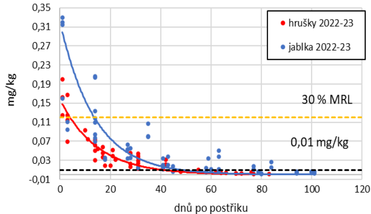
mefentrifluconazole
